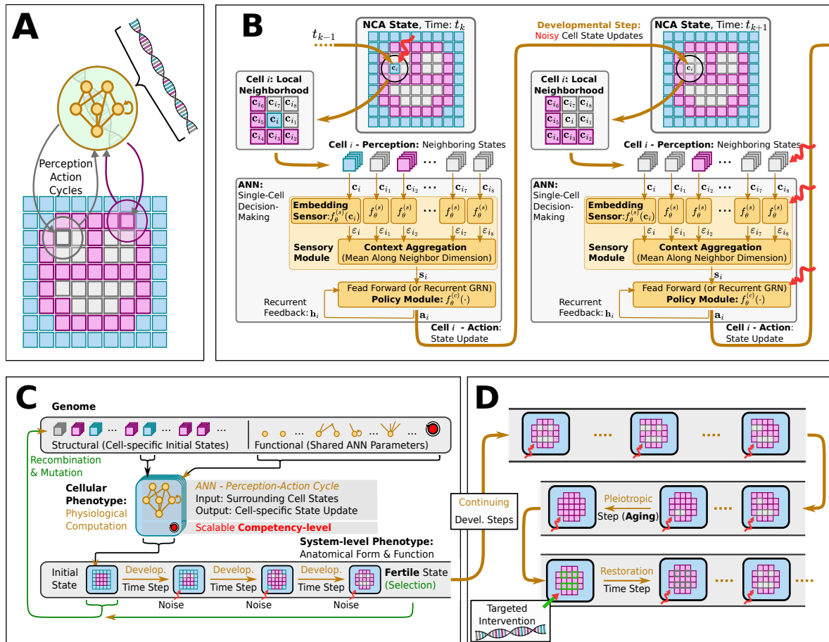
Figure 2. (A): Schematic computational model of a biologically inspired multi-scale competency architecture [1], relying on Neural Cellular Automata [2,3] (NCAs) in an evolutionary setting [4]: in an evolutionary NCA, a genetic code, i.e., a cell's "DNA" (represented by a string of numerical parameters), is compiled into a uni-cellular phenotype containing a proto-cognitive decision-making center (represented by a tiny recurrent neural network parameterized by the "DNA") by which the cellular agent can actively regulate its own numerical cell state based on local measurements of the states of its immediate cellular neighbors on a square grid of cells. In that way, the collective of cells can be trained, or evolved, to perform morphogenesis of a predefined target pattern of expressed cell types (color-coded in blue, magenta, and white), of, e.g., a smiley-face pattern (reminiscent of the bioelectric craniofacial prepattern defining the amphibian face [5]). (B): Detailed information flowchart of uni-cellular decision-making of cells on the grid of a NCA, modeling the process of morphogenesis (c.f., (A)): each cell expresses its cell-type based on local communication protocols with its neighboring cells so the collective of cells self-assembles a target pattern. This is implemented via subsequent uni-cellular perception-action cycles that update each cell's respective state on the NCA's grid purely based on local measurements of neighboring cell states. (C): Schematics of the evolutionary process of uni-cellular competencies that drive the self-orchestrated morphogenesis of a target pattern (here, of a smiley, face). (D): Schematics of long-term behavior of an NCA evolved in (C) that is not controlled by the evolutionary process. Developmental errors or noise (red wiggly arrows) might lead to a collapse of the target pattern over time, especially long after the selection process occurs (where genetic material is passed on to the next generation. Following pleiotropic considerations, we assume that the long-term "solutions" or the target morphogenetic state might significantly differ from the target state that the evolutionary process "sees" through selection, simply because different states might be more probable (such as, here, a "red" circle without facial features). Moreover, detecting such deviating pleiotropic defects (missing facial features, in our case), and performing targeted interventions of the most affected cells allow us to "reprogram" the cellular collective and reset it via targeted interventions - without further optimization or adaptation - so the tissue auto-regenerates to the original target pattern.
