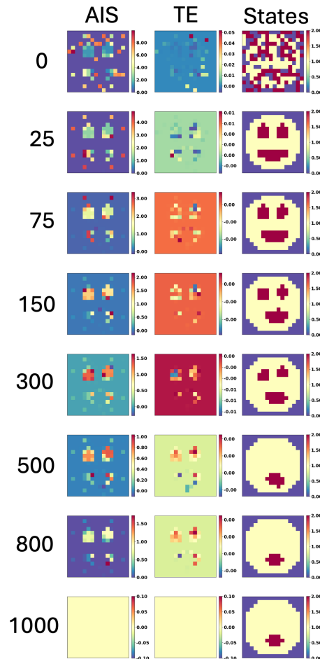
Figure 7. . Loss of the organs but not of the information about the organ during normal aging. In order to study the information dynamics during aging and morphological decay, we applied AIS and TE during development and aging. Here is an example of a morphogenetic experiment where the organism is losing organs, here the eyes of the smiley face at step 500 in States column. But both AIS and TE are high at the spatial location of these organs (from 500 to 800 steps). This suggests memory retention, similarly to regenerative organisms that can regrow lost organs or limbs, keeping some memory of the lost body parts. This result will lead to the organ regeneration experiment (see Figure 8).
