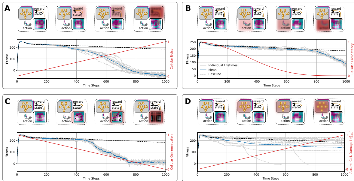
Figure 5. Panels (A–D): Schematic visualization of the amplified damaging processes to cellular competencies corresponding to Sections 4.1.3–4.1.6, respectively. (A): The fitness over the lifetime of the 16 \times 16 smiley-face NCA discussed in Section 3 where the noise level for cell-state updates is linearly increased from \zeta_c(t_k = 0) = 0 to \zeta_c(t_A) = 1 (emphasized by red line), for t_A = 1000 time steps t_k ; gray lines show statistically independent trajectories of individual lifetimes of the NCA, the blue line represents the corresponding ensemble mean, and the black-dashed line is the baseline mean fitness without corrupted competencies (c.f., Figure 4). (B): similar to (A) but corrupting cellular competencies via a successively decreasing decision-making probability P_D(t_k = 0) = 1 to P_D(t_A) = 0 following the functional form P_D(t_k) = \sin\left[\frac{\pi}{2}\left(1 - \frac{t_k}{t_A}\right)\right]^4 (see red line). (C): similar to (A, B) but permanently corrupting the intercellular communication pathways by successively disabling randomly selected communication channels (reminiscent of gap-junctions [44]) between neighboring cells by linearly decreasing the gap-junction prohibiting probability from P_{GJ}(t_k = 0) = 1 to P_{GJ}(t_A) = 0 (see text and red line). (D): similar to (A–C) but accumulating genetic damage in the unicellular decision-making machinery, i.e. , corrupting intracellular information processing and decision-making by adding zero-centered Gaussian noise of standard deviation \sigma_x = 10^{-2} at every time step to the cells’ ANN parameters (which is equivalent to ANN parameters corrupted by \sigma_x^2(t_k) = t_k \sigma_x^2 at time-step t_k with \sigma_{\max}^2 = \sigma_x^2(t_A) ). In (A–D), the top panels schematically illustrate the perception-action cycles of every cell over the lifespan of the NCA; the particular processes affecting the cellular competencies, thus enhancing the rate of degradation of the target pattern in each panel (A–D), are emphasized from left to right by panel (A–D) by red blurry blocks: this involves (A) increasingly noisy cell states directly affecting the NCA’s state perception, (B) increasingly unreliable cell decisions directly affecting the NCA’s action output, (C) successively corrupted intercellular communication channels directly affecting the exchange of information between neighbors, and (D) accumulation of genetic damage by successively diffusing the cells’ ANN parameters directly affecting the unicellular decision-making machinery.
