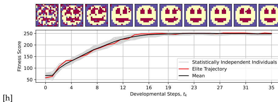
[h] Figure 3. Typical fitness score evaluations during t_D = 35 developmental steps of morphogenesis of 50 statistically independent runs of an NCA that has been evolved to self-assemble a (16 \times 16) -smiley-face pattern. Example NCA states from the individual with the highest developmental fitness score (c.f., red “elite trajectory” in bottom panel) are presented throughout the developmental phase as temporal snapshots corresponding to the ticks of the horizontal axis; background-, facial-, and internal organ cells (of eyes and mouth) are colored purple, yellow, and red, respectively.
